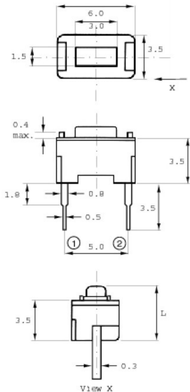
PCB Mounting Holes - Straight Leads
